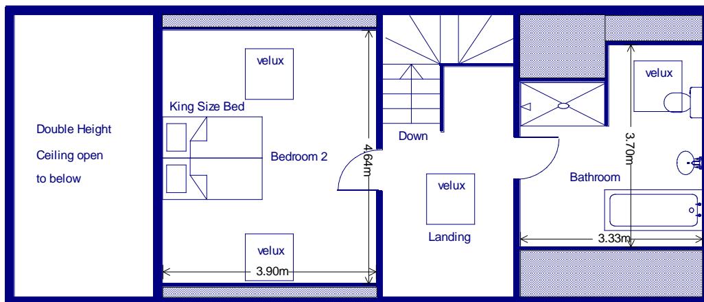
1st Floor
